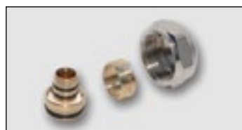
Art. H-LINE.1039.1620 H-LINE adaptér G 3/4" x 18 (EUROCONUS) na Al-Pex, Pex, Pert trubky 16 x 2
